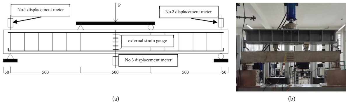
FIGURE 3: Layout of measuring points and loading device diagram. (a) Layout of measuring points. (b) Loading device.
