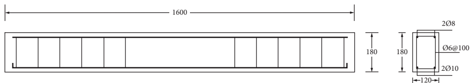
FIGURE 2: Size and reinforcement diagram of the test beam (unit: mm).
