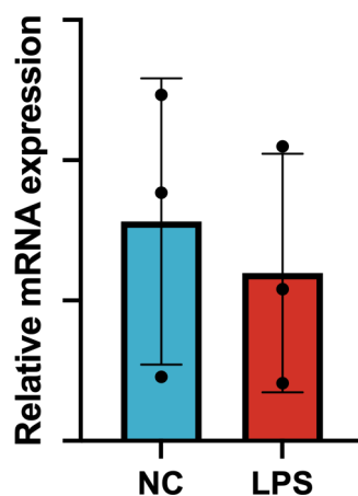
BSN
