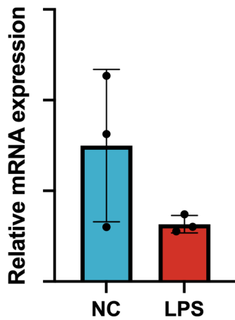
SLC6A4
