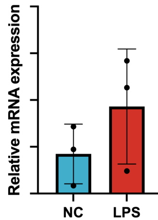
SLC2A4
