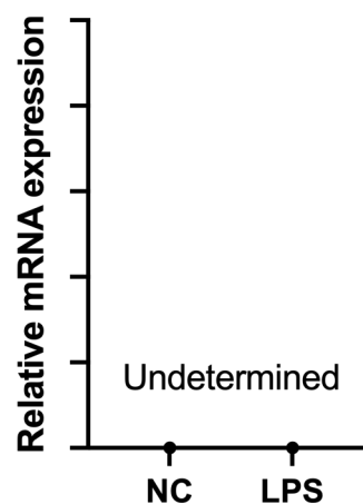
PRKG1
