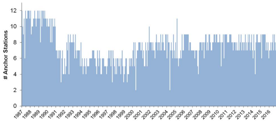
Figure 1 – Supplementary Material: Number of anchor stations used for the estimation of CHIRPS dataset in the domain 31°-39°S; 67°-71°W. Period 1987-2016.
