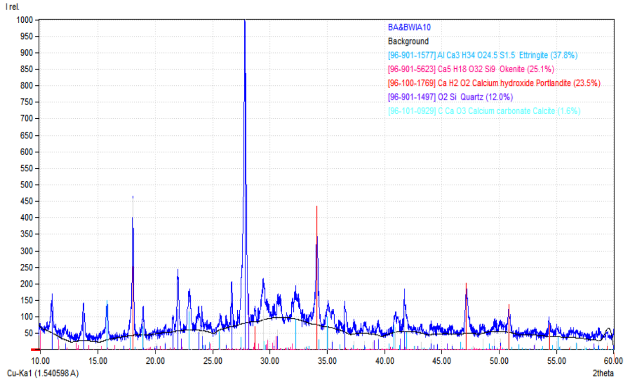
Figure 3:-Diffraction Pattern Graphics of 5% BA and 5% of BWIA mix (BA&BWIA 10)
