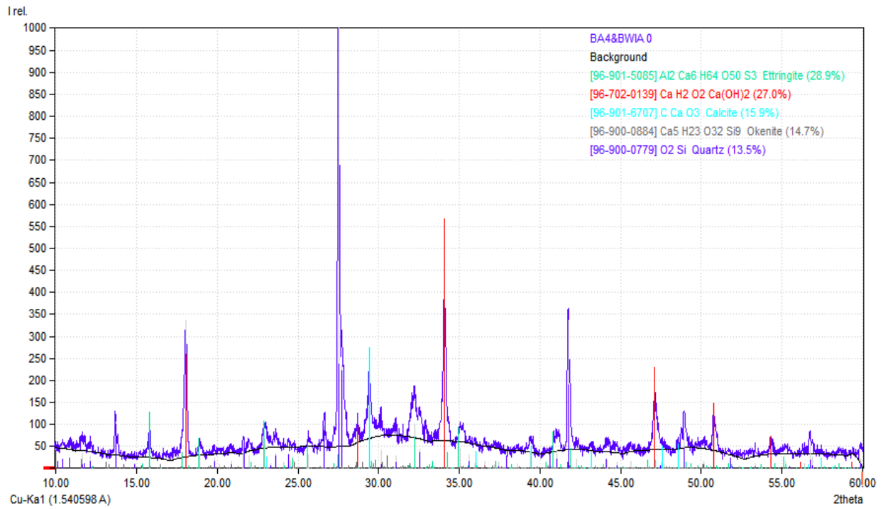
Figure 1:- Diffraction Pattern Graphics of control mix (BA and BWIA 0)
