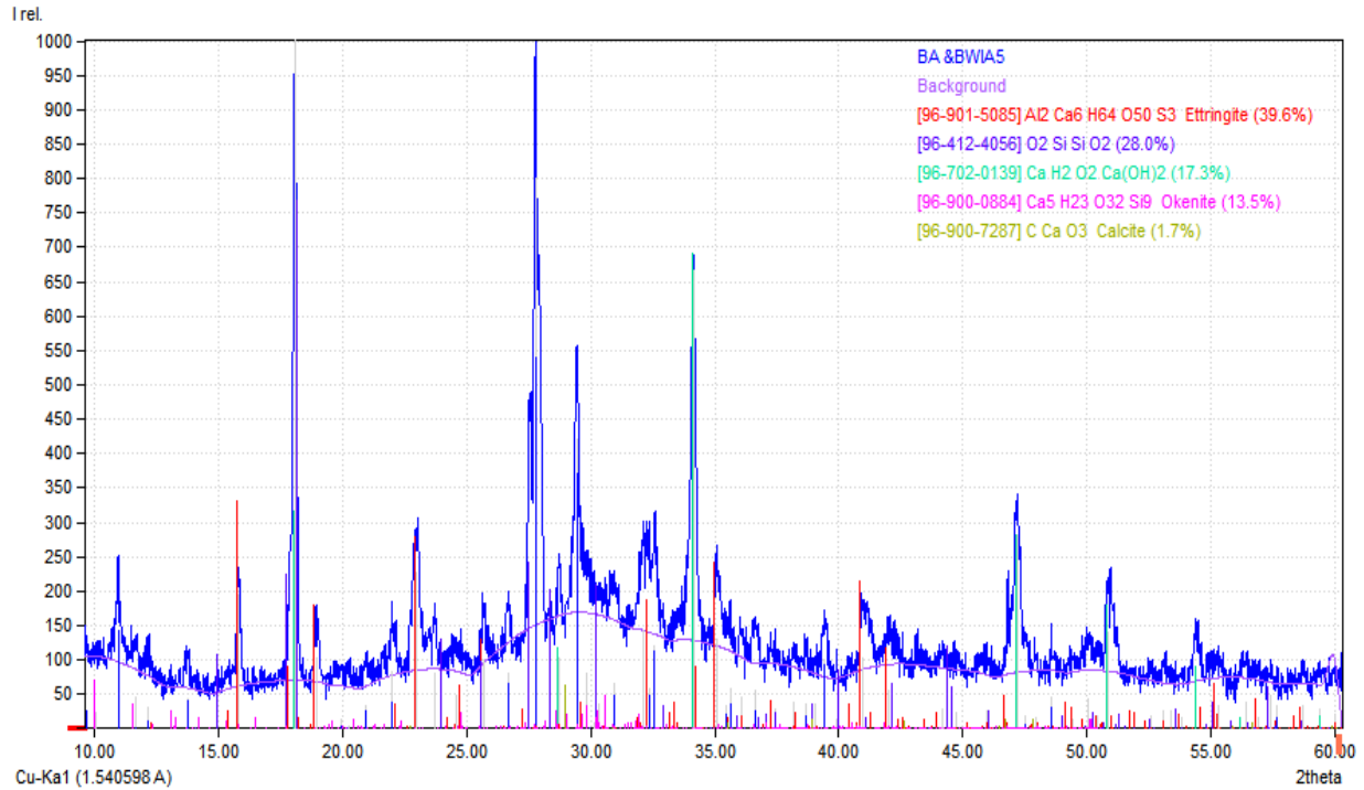
Figure 2:-Diffraction Pattern Graphics of 2.5% BA and 2.5% of BWIA mix (BA&BWIA 5)
