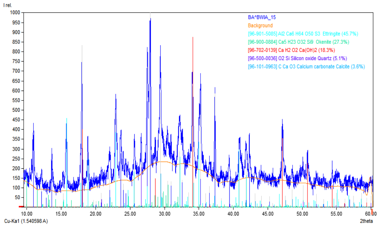
Figure 4:-Diffraction Pattern Graphics of 7.5% BA and 7.5% of BWIA mix (BA&BWIA 15)
