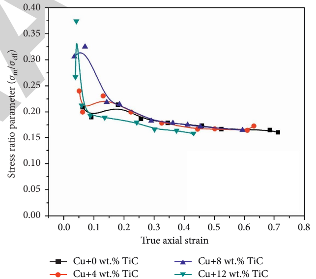
FIGURE 17: Stress ratio parameter ( \sigma_m/\sigma_{eff} ) versus true axial strain ( \epsilon_z ).
