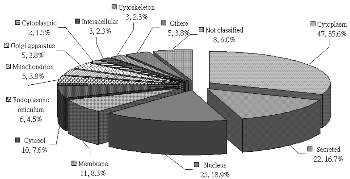
Figure S2. The cellular locations of 132 proteins synthesized were classified in this study. Assignments were made on the basis of information provided on the Swiss-Prot database at the ExPASy Molecular Biology Server. Some proteins were described to be from a different subcellular location, which explains the total sum being substantially larger than 100%.
