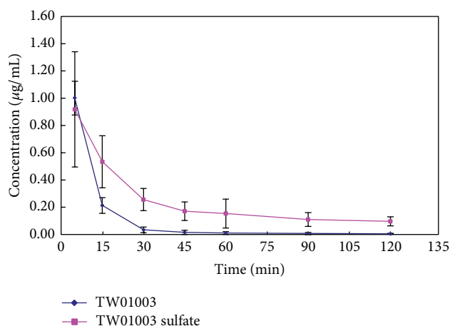
FIGURE 5: Plasma concentration-time profile of TW01003 and TW01003 sulfate after i.v. administration of TW01003 ( n = 6 ).
