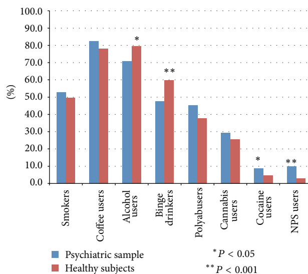
FIGURE 1: Psychoactive substances.
