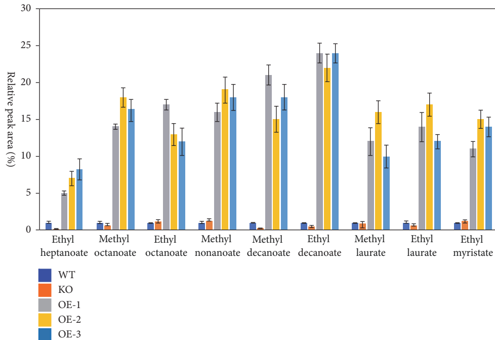
FIGURE 8: Production of volatile compounds in WT, KO, and three lines of OE measured by SPME GC-MS. Strains were allowed to ferment for 24 h at 30°C, and volatile compound production was subsequently induced with 0.5 % methanol for 48 h. Amounts of individual volatile compound are shown as percentage of total aromas. Data represent the mean from triplicate experiments \pm standard deviation.
