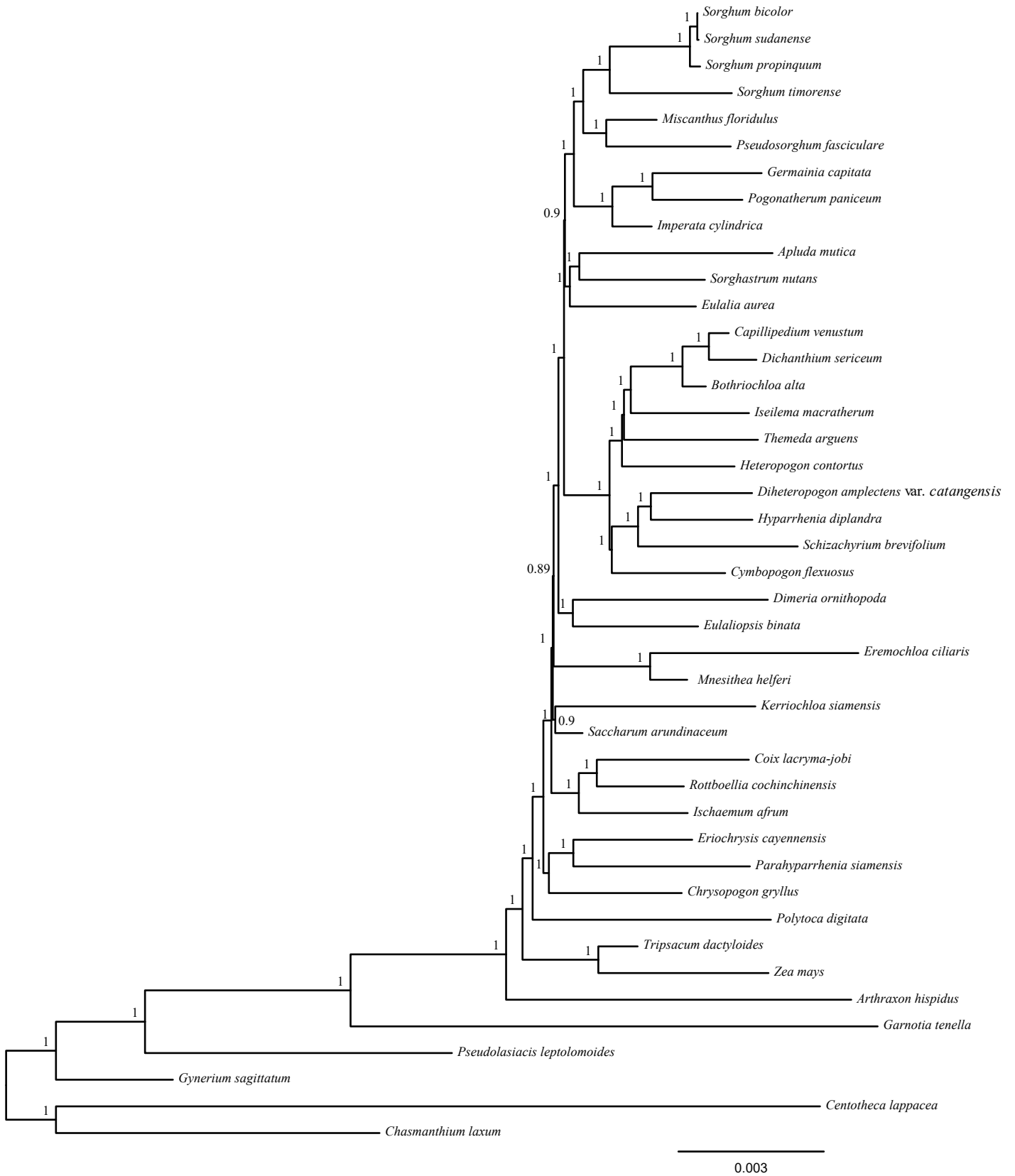
Figure S1. Phylogenetic relationships of the Andropogoneae species constructed from the complete chloroplast genome sequences using Bayesian inference (BI).
