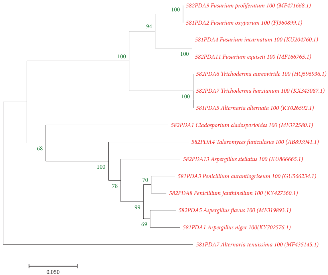
FIGURE 2: Phylogenetic tree constructed with ITS-rDNA sequences of fungal endophytic isolates obtained from tissue sections of wheat using neighbor-joining method. Evolutionary analyses were conducted in MEGA7.
