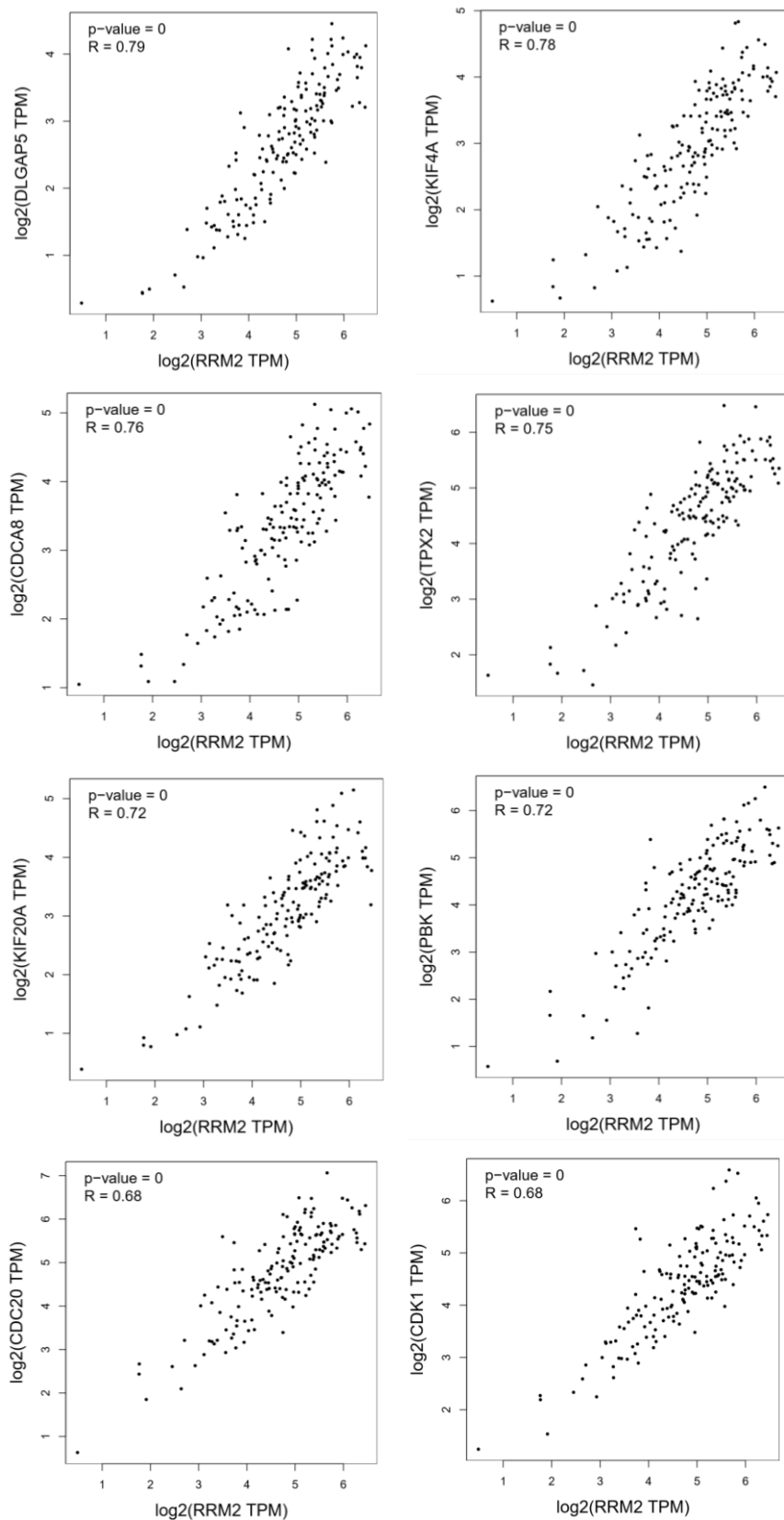
Supplementary Figure 1. Correlation between the expression of RRM2 and other hub genes.
