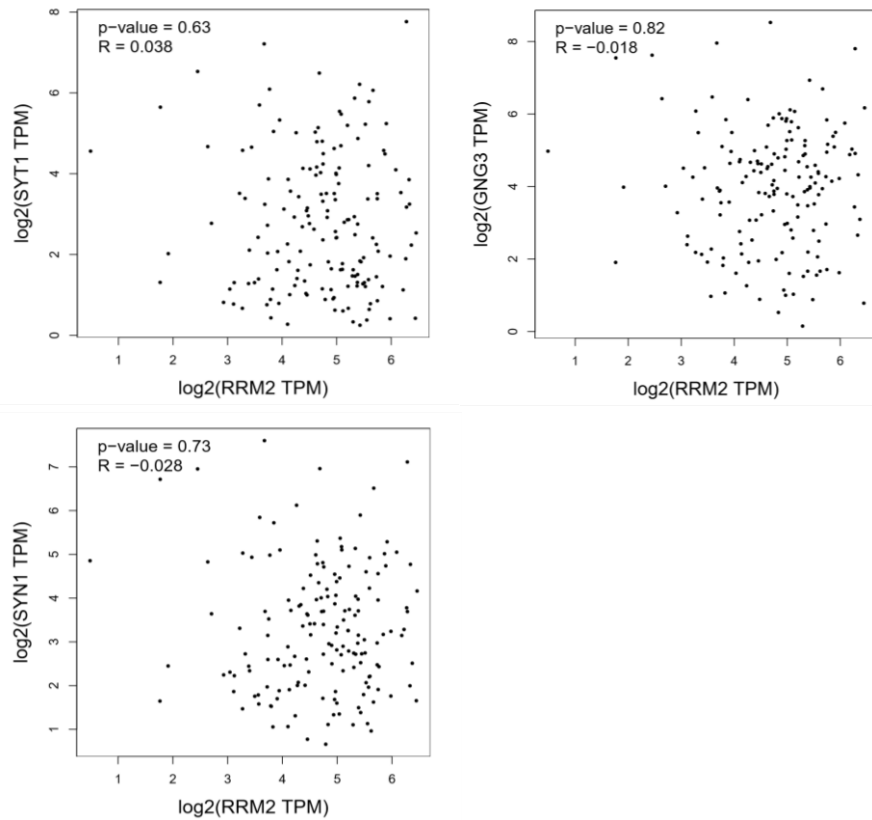
Supplementary Table.1 Correlation between the expression of RRM2 and other hub genes.
