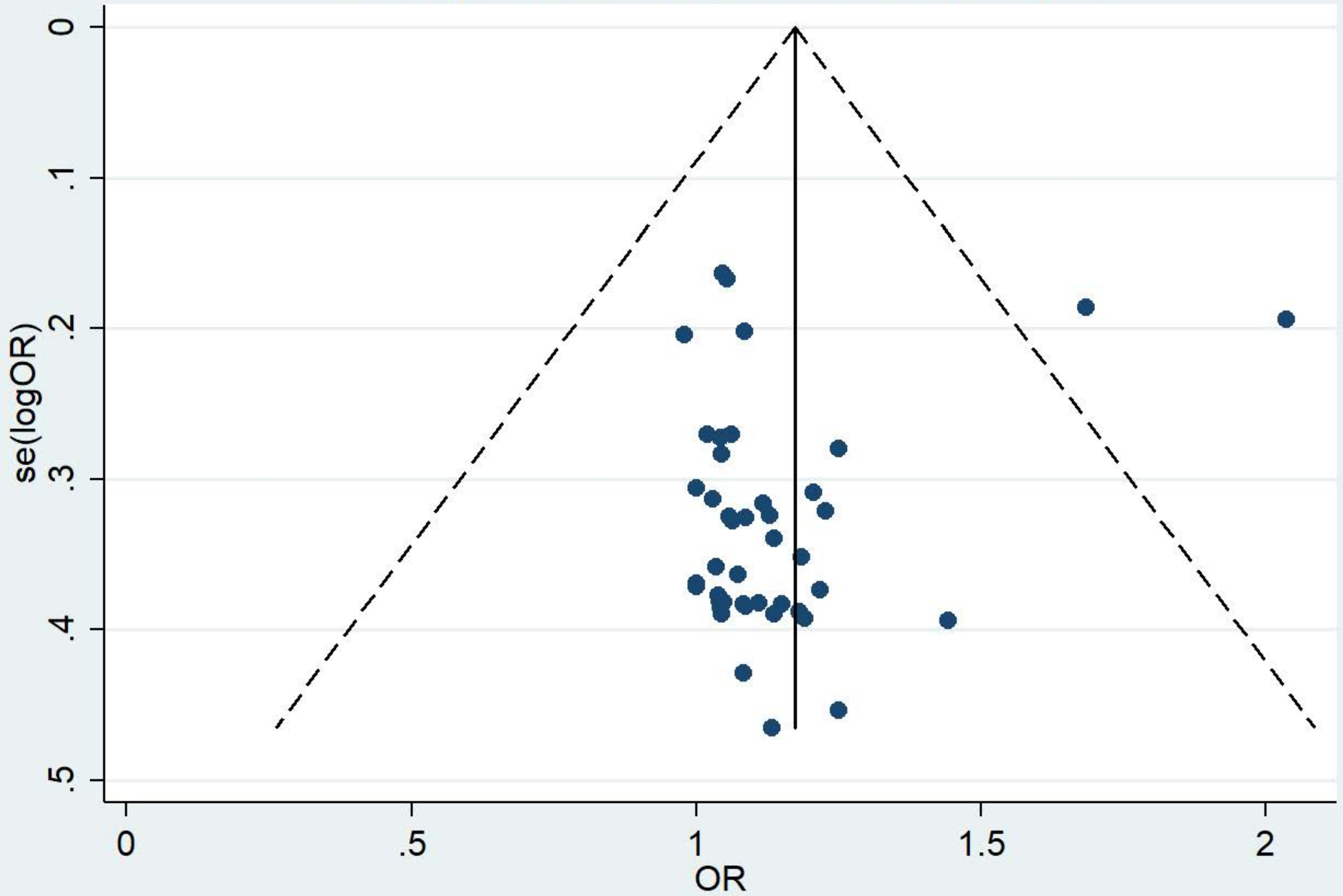
Funnel plot with pseudo 95% confidence limits
