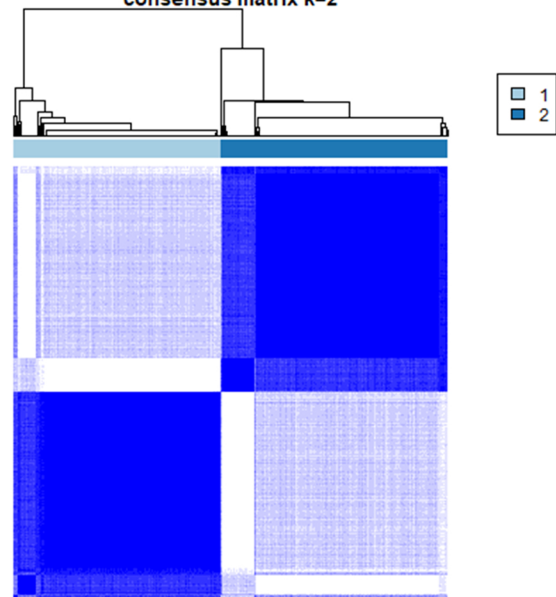
consensus matrix k=2
