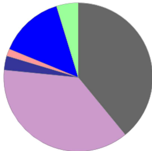
Molecular Function
