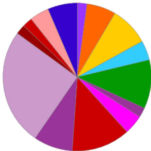
Protein Class
