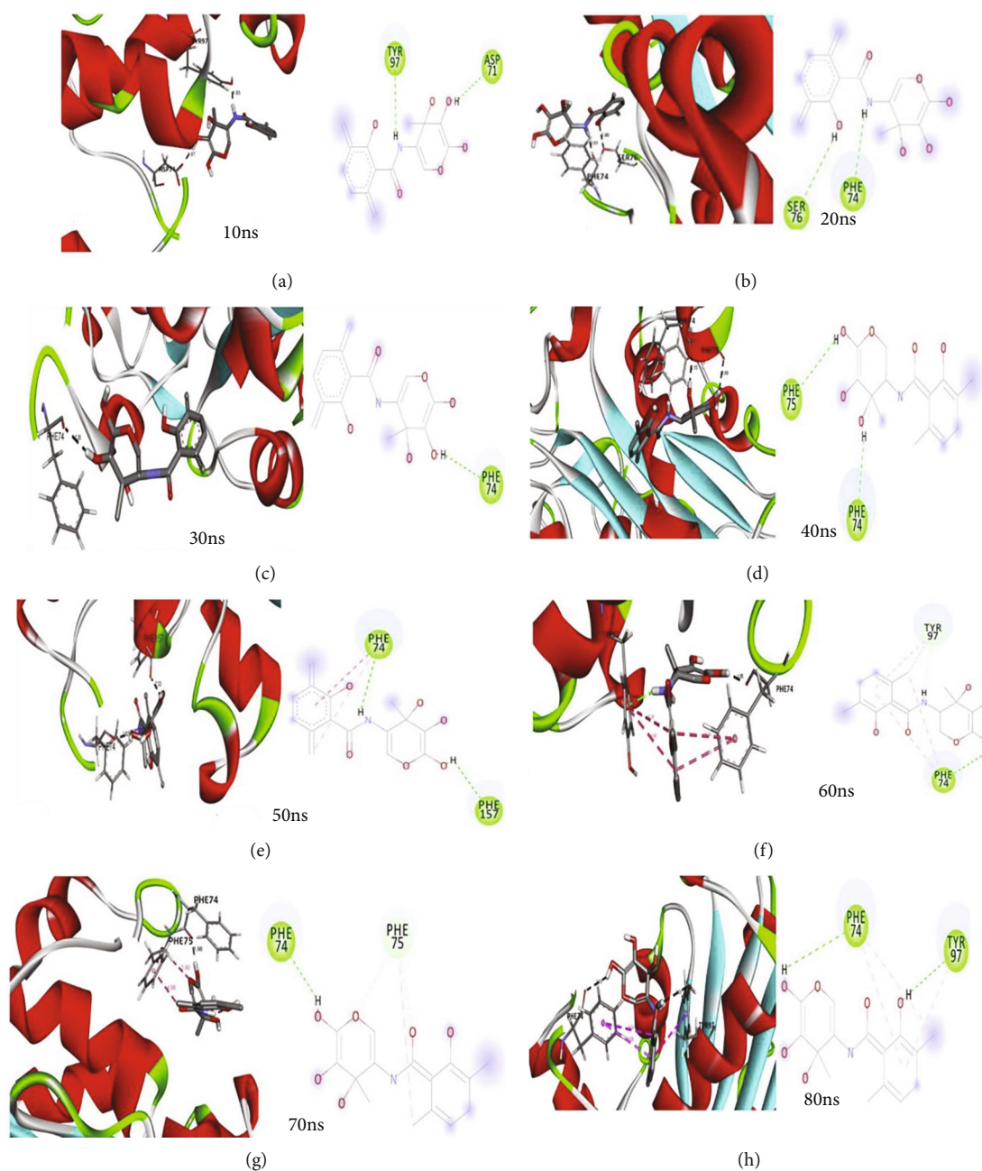
FIGURE 7: (a–h) Three-dimensional (3D) and two-dimensional (2D) interactions of polyketide synthase beta-ketoacyl synthase domain-CMNPD24498 at different time slots during MD simulation.
