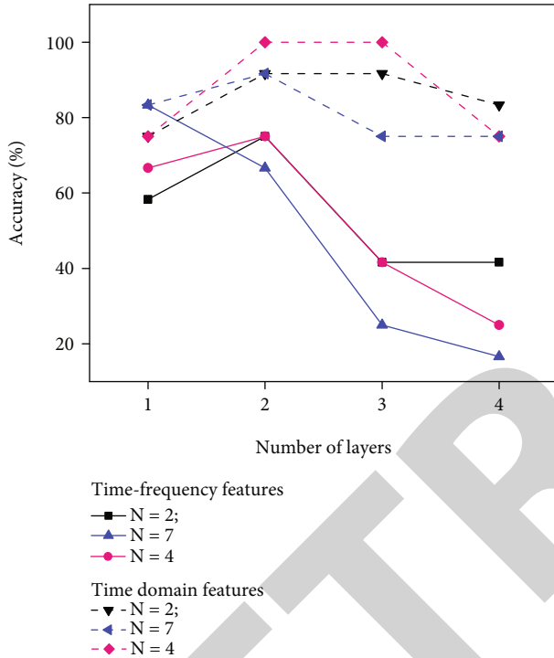
FIGURE 4: Accuracy of CANN and DNN classifiers of different hidden layers and hidden neurons for time and time-frequency features.
