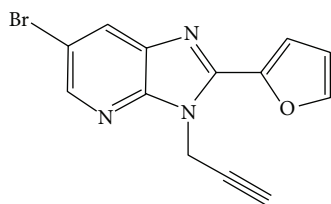
SCHEME 1: Compound 1.
