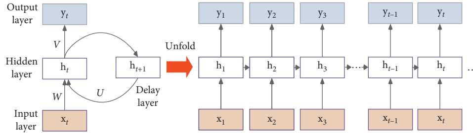
FIGURE 1: Architecture of RNN unfolded in time.
