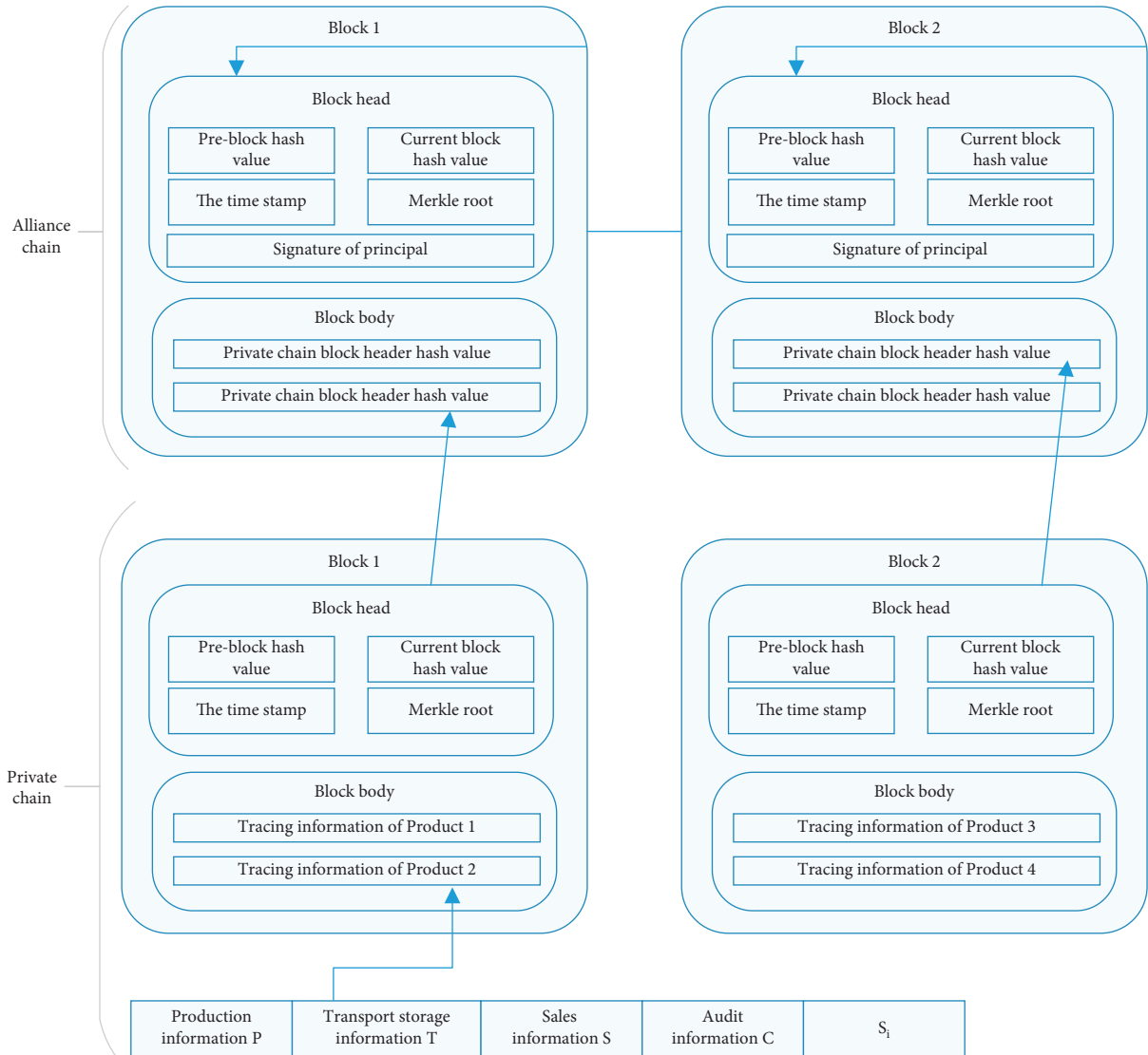
FIGURE 3: Data structure of private chain and alliance chain.
