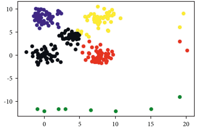
FIGURE 1: The k -means ++ clustering result on synthesized dataset.
