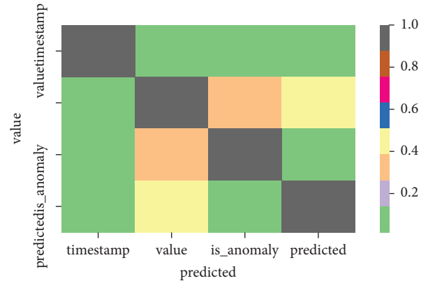
FIGURE 5: Generated matrix.
