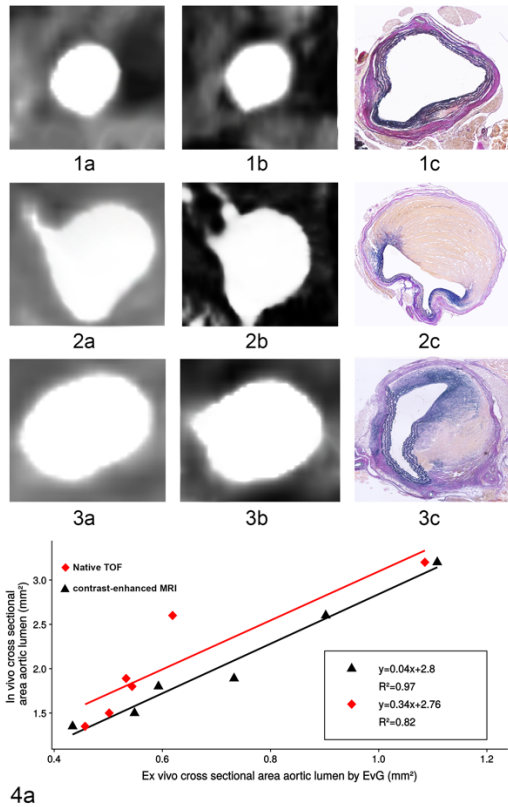
Supplementary Figure 1: Visualization of an abdominal aortic aneurysm (AAA) and in ApoE -/- knockout mouse by MR angiography on a clinical 3T MR system. Images demonstrate the visualization of AAA by in vivo MR angiography on a clinical 3T MR system. Non-contrast-enhanced MR angiogram (TOF, a) and contrast-enhanced MR angiogram (GdT, b) in direct comparison to the associated histology of the arterial vessels (c). A strong correlation between in vivo and ex vivo measurements was measured (4a).
