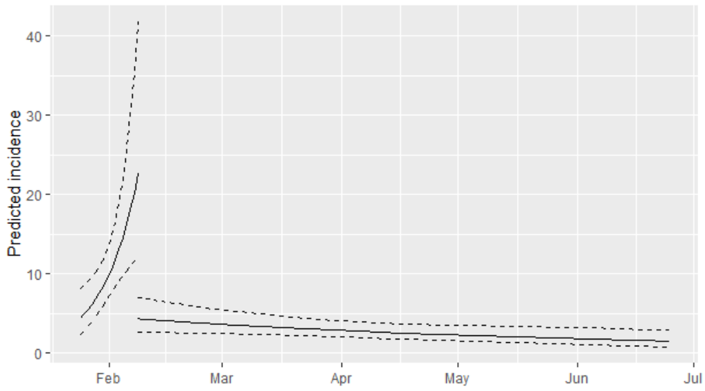
Figure 1: Fitted Prediction Models with Intervals for Infections in Hebei Province, China
