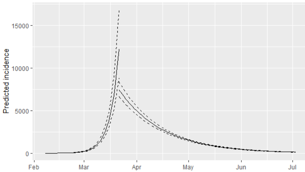
Figure 2: Fitted Prediction Models with Intervals for Infections in Italy
