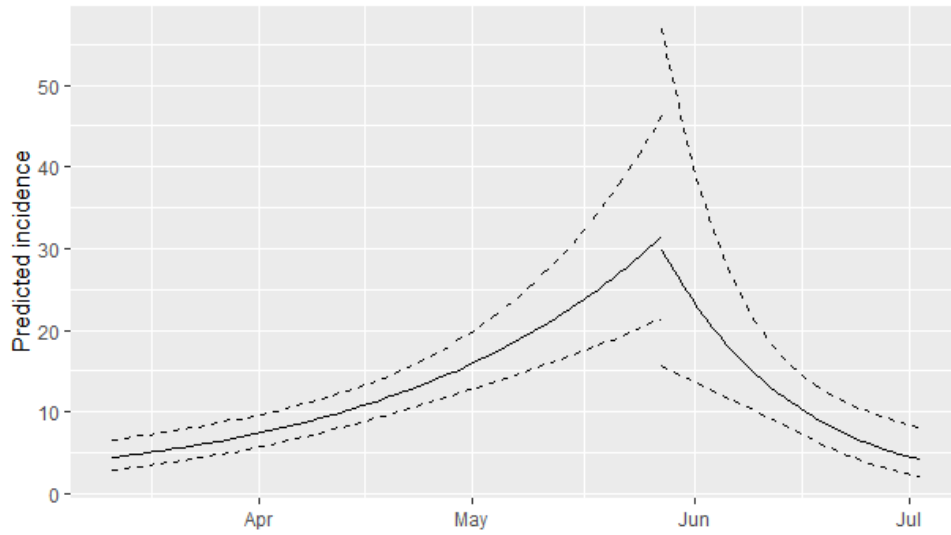
Figure 3: Fitted Prediction Models with Intervals for Infections in Sri Lanka
