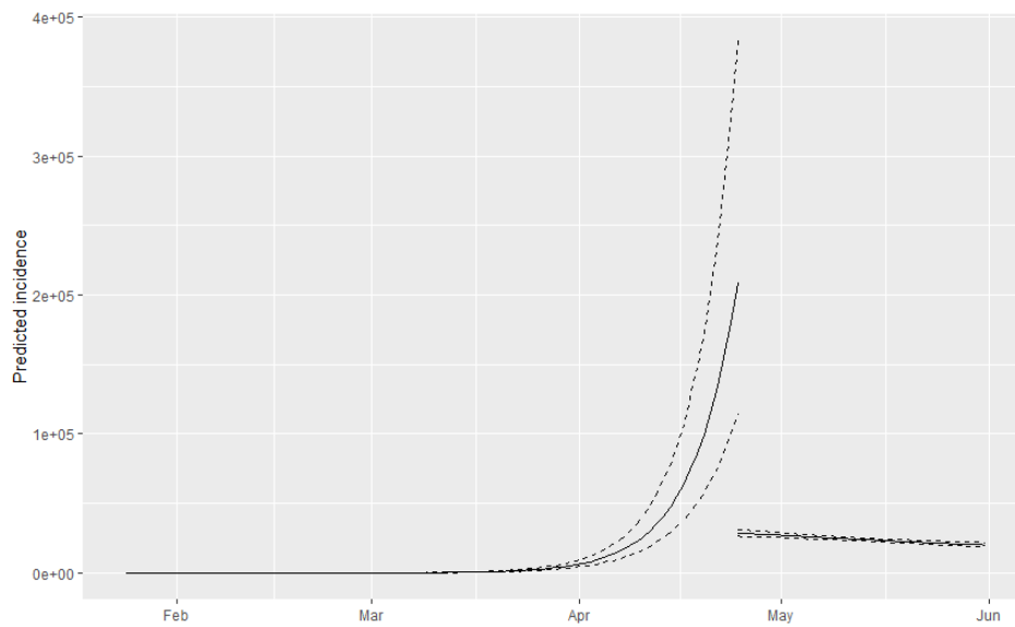
Figure 4: Fitted Prediction Models with Intervals for Infections in United States – First Data Set
