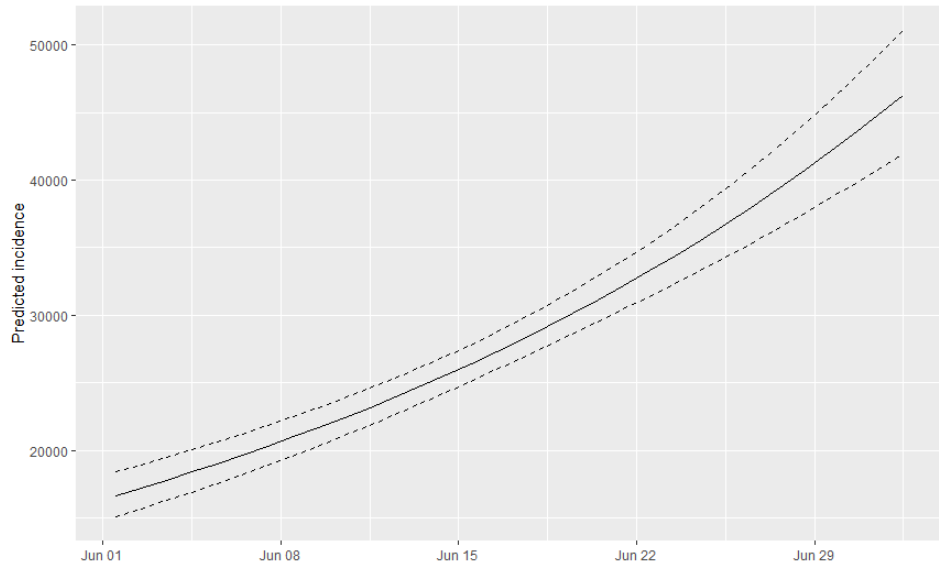
Figure 5: Fitted Prediction Model with Interval for Infections in United States – Second Data Set
