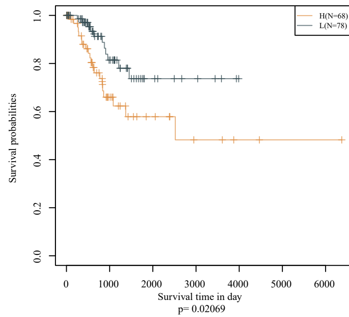
ARMCX1
