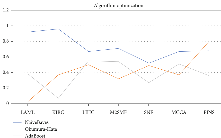
FIGURE 7: Algorithm optimization.
