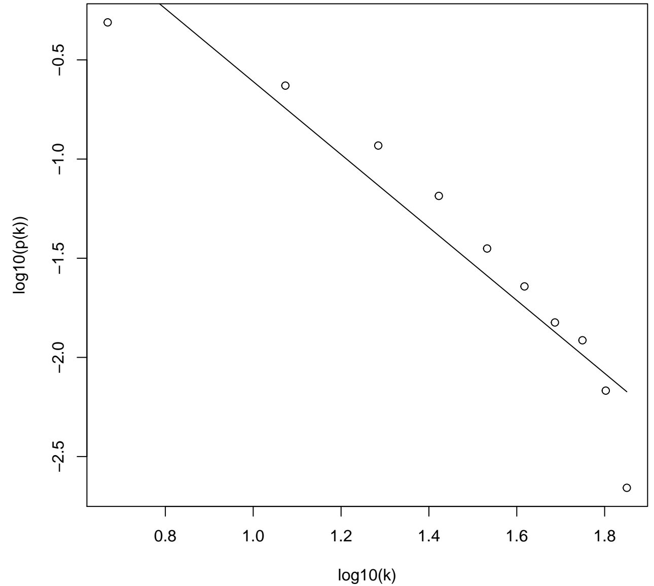
Check scale free topology scale R^2= 0.89 , slope= -1.84
