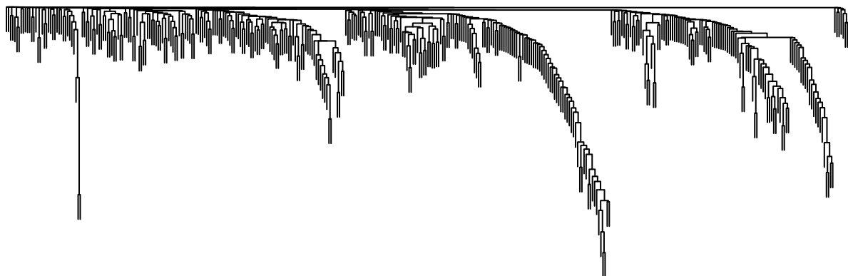
Network heatmap plot, select 400 genes
