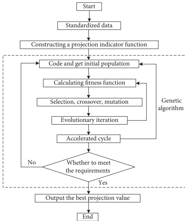
FIGURE 1: RAGA-PP model flowchart.
