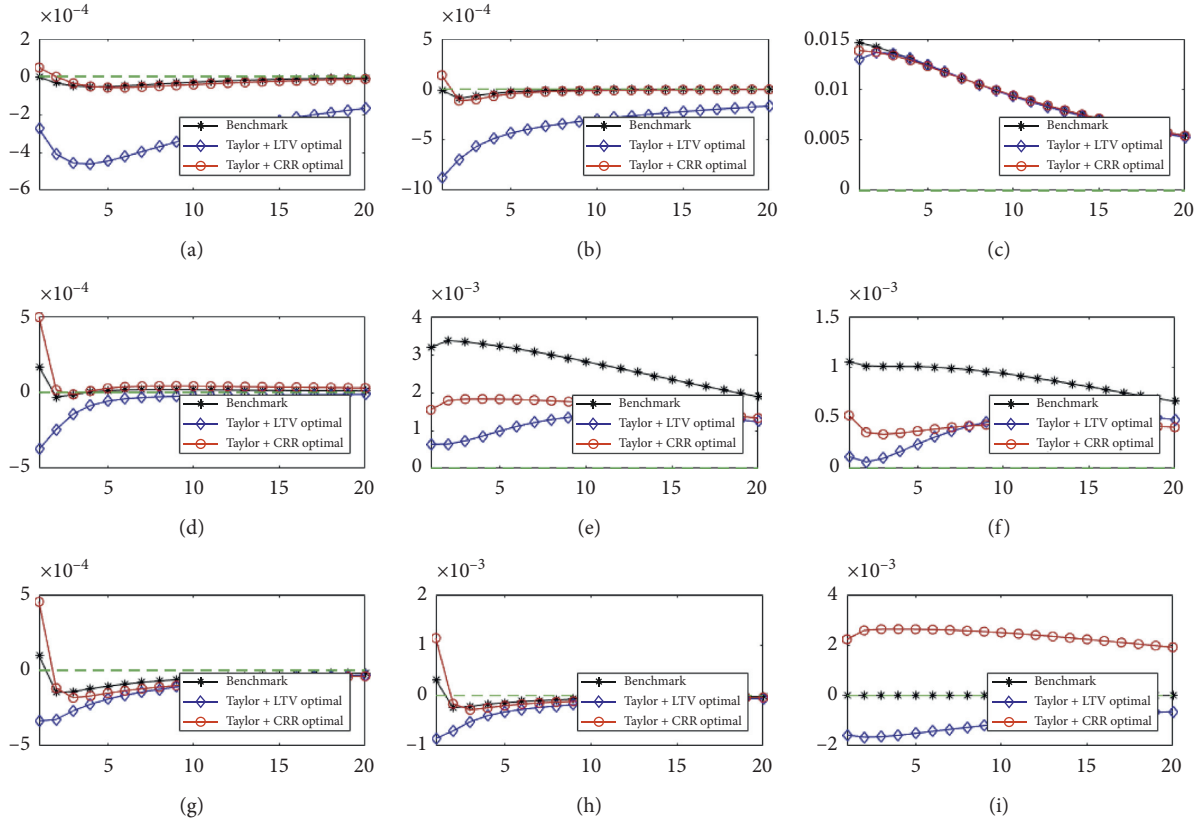
FIGURE 1: Impulse response analysis of a housing preference shock. (a) Rs, (b) Pai, (c) q, (d) y, (e) bb, (f) Hb, (g) Cb, (h) Wb, and (i) kappa CRR.
