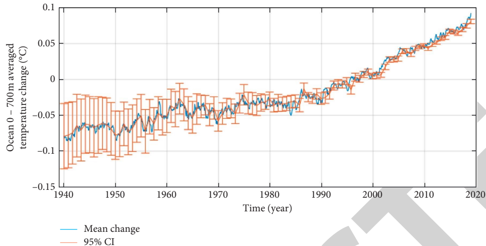
FIGURE 1: The map of global ocean average temperature change.
