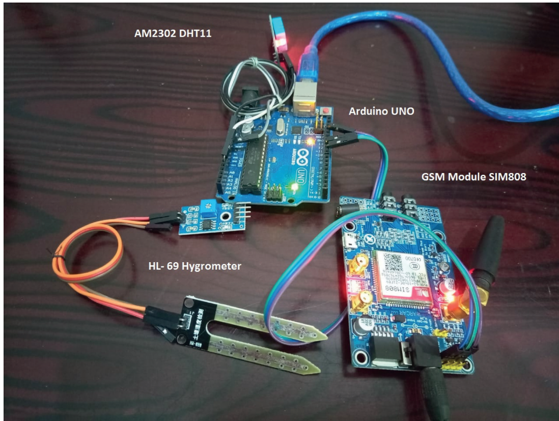
FIGURE 5: Hardware prototype.
