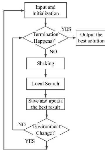
Figure S1: The flowchart of VNS.
