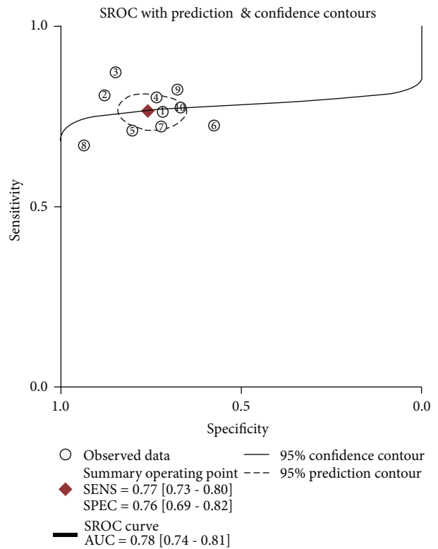
FIGURE 5: Summary receiver operating characteristic curve for circRNAs in diagnosing lung cancer.
