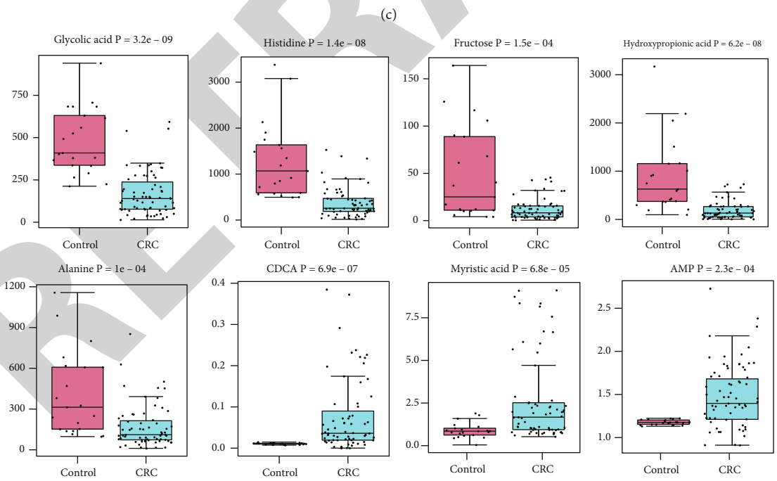
FIGURE 3: Differential metabolites for CRC urine sample compared to control. (a) Volcano plot for differential metabolites identified by OPLS-DA in CRC patients vs controls (VIP>1, |correlation coefficient|>0.3). (b) Volcano plot for differential metabolites identified by univariate statistical analysis in CRC patients vs controls ( p < 0.05 , significantly increased metabolites in CRC (FC>1, red dots) and significantly decreased metabolites in CRC (FC<1, blue dots). (c) Heatmap of differential biomarkers of CRC patients vs controls (Z-score scale to -2~2). (d) Box plot of representative differential metabolites with significantly different concentration in CRC sample vs control ( p < 0.05 ).
