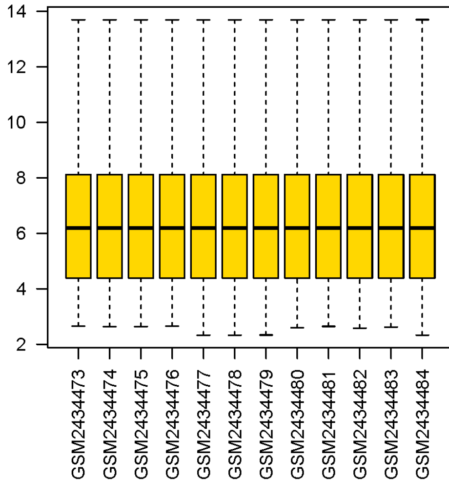
Boxplot for GSE92681
