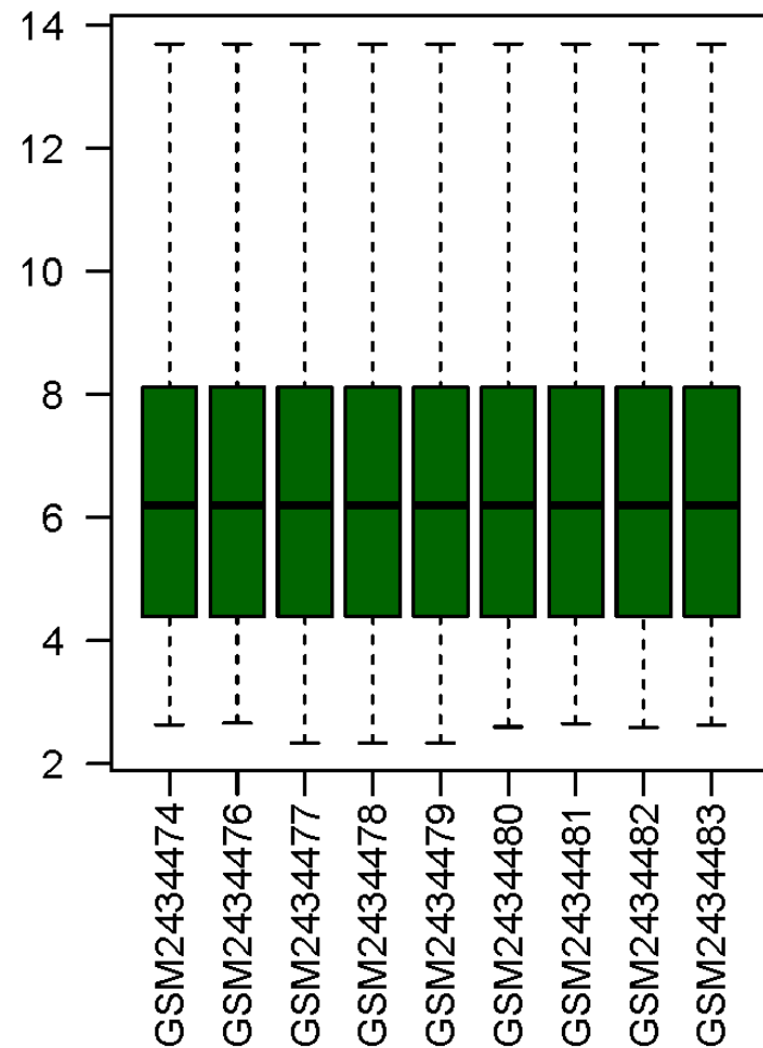
Boxplot for GSE92681 after removing outliers
