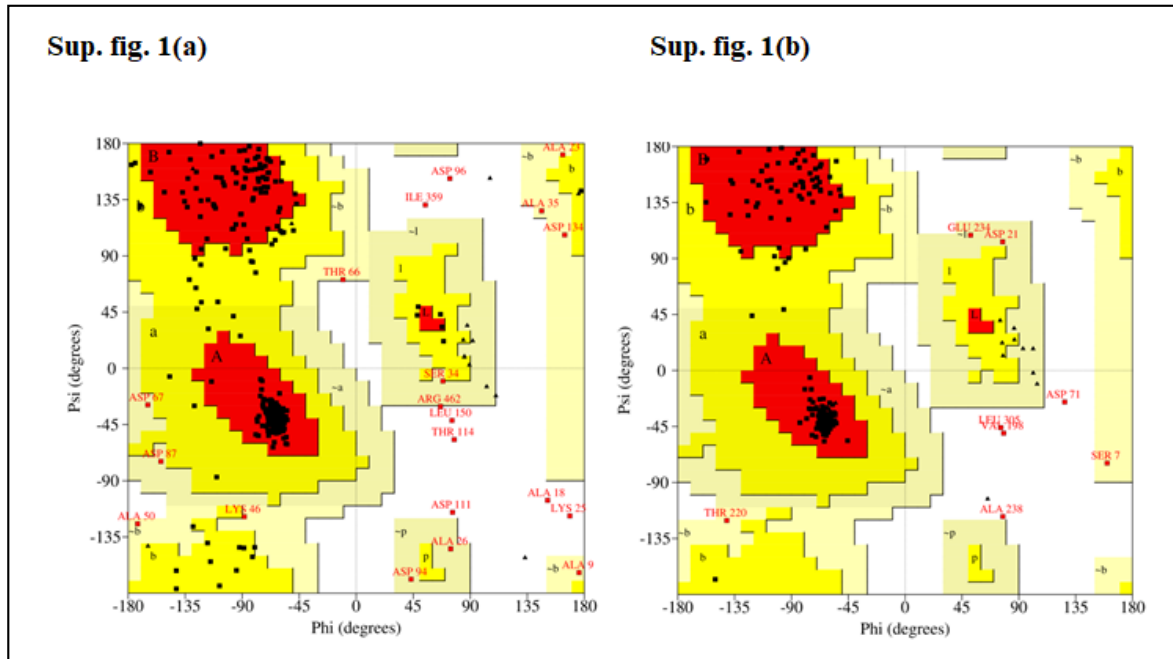
Sup. fig. 1: Ramachandran plots for the homology models of a) M. smegmatis SigA and b) M. smegmatis SigB
