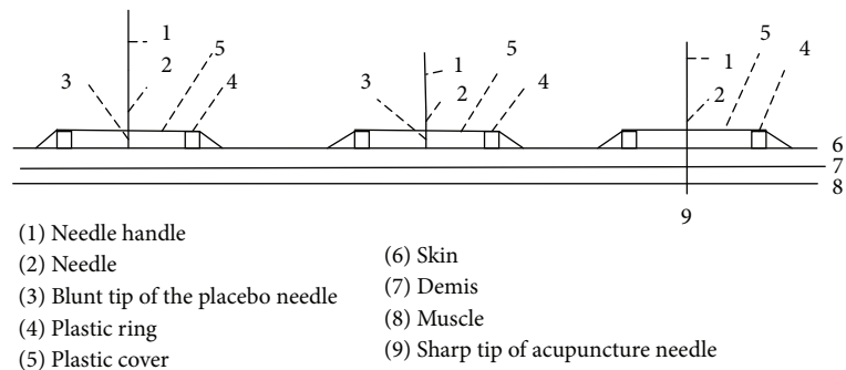
FIGURE 1: Placebo needle.
