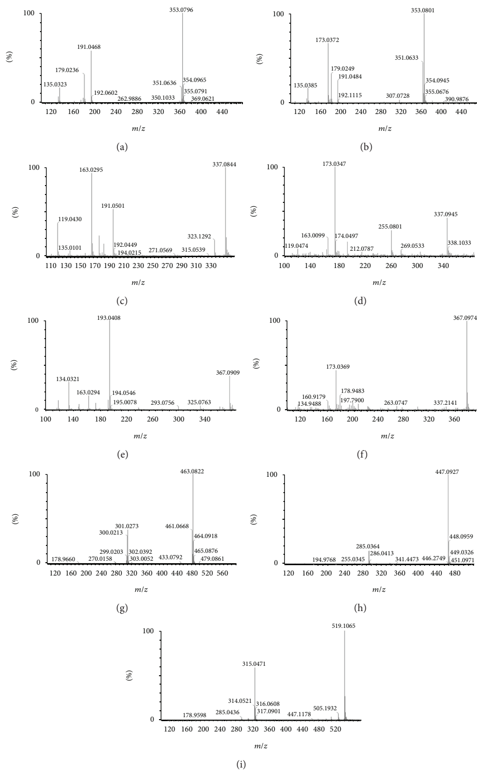
FIGURE 3: The representative UPLC-QTOF-MS spectra showing fragmentation patterns of 3CQA (a), 4CQA (b), 3pCoQA (c), 4pCoQA (d), 3FQA (e), 4FQA (f), quercetin-O-glycoside (g), kaempferol-O-glycoside (h), and isorhamnetin-O-glycoside (i) generated at a collision energy of 30 eV.
