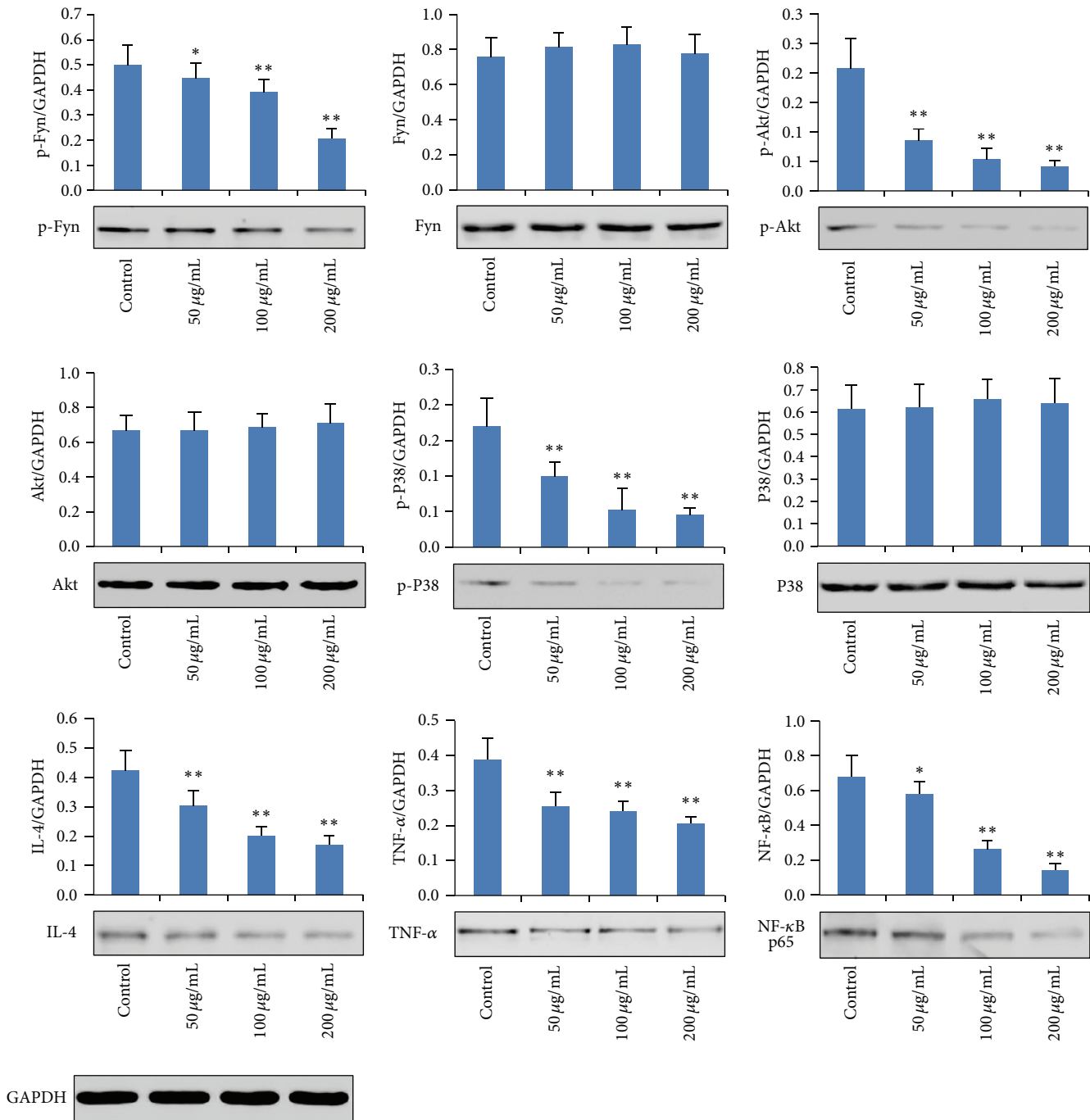
FIGURE 4: Effects of AP on protein expressions of p-Fyn, Fyn, p-Akt, Akt, p-P38, P38, IL-4, TNF- \alpha , and NF- \kappa B p65. Data are represented as mean \pm SD ( n = 6 ), * p < 0.05 , and ** p < 0.01 , compared with control group.
