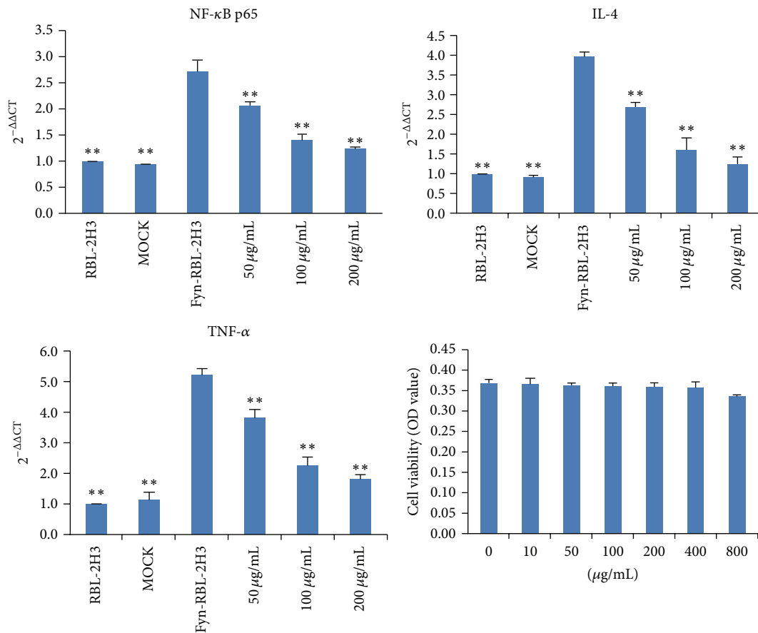
FIGURE 6: Effects of AP on mRNA expressions of NF- \kappa B p65, IL-4, and TNF- \alpha in upregulated RBL-2H3 cells stimulated with anti-DNP IgE. MOCK means the cells treated with control vector, and Fyn-RBL-2H3 means Fyn gene upregulated RBL-2H3 cells, ** p < 0.01 , compared to Fyn-RBL-2H3 cells.
