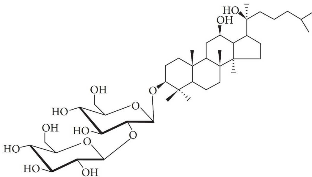
Supplemental Figure 1: The chemical structure of Rg3.
