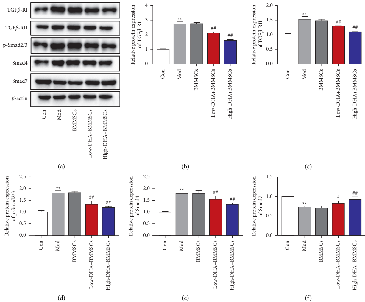
FIGURE 5: DHA inhibited TGF- \beta /Smad signaling pathway in CBP mice. (a) Representative bands of Western blot analysis. Expression of TGF- \beta -RI (b), TGF- \beta -RII (c), p-Smad2/3 (d), Smad4 (e), and Smad7 (f) in the prostatic tissues of mice was detected by Western blot. **denotes P < 0.01 vs con group, # denotes P < 0.05 vs BMMSCs group, and ## denotes P < 0.01 vs BMMSCs group. For (b)–(f), mean \pm standard errors of means are reported.
