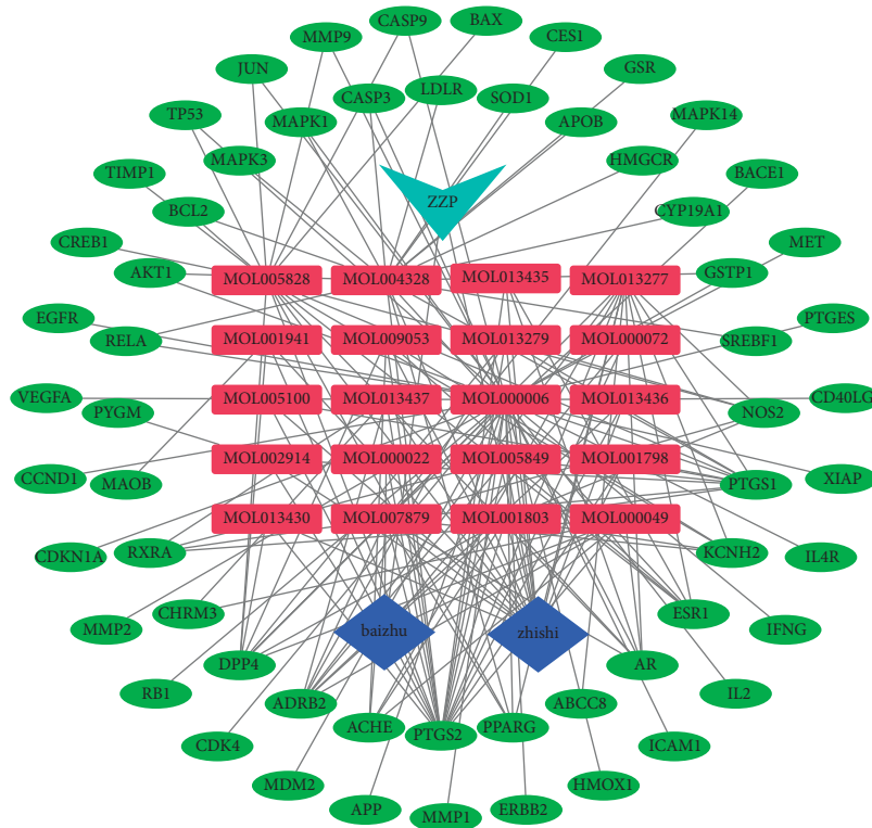
FIGURE 3: Drug-compound-target gene network of ZPP. The red squares represent the components; the green ellipses represent targets; purple diamonds represent different herbs; and blue arrows represent ZPP. The edges represent the relationship between the components and the targets.
