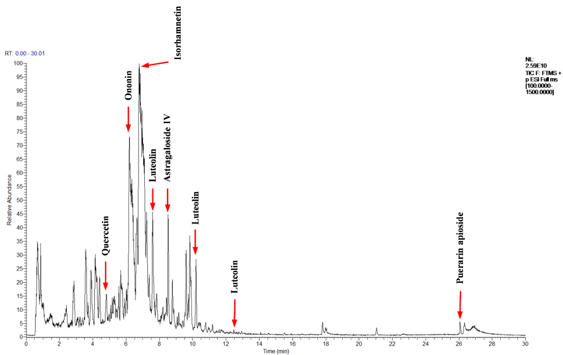
TIC diagram of UHPLC-Q Exactive-MS detection of YJHD granule aqueous solution in positive ion mode.
