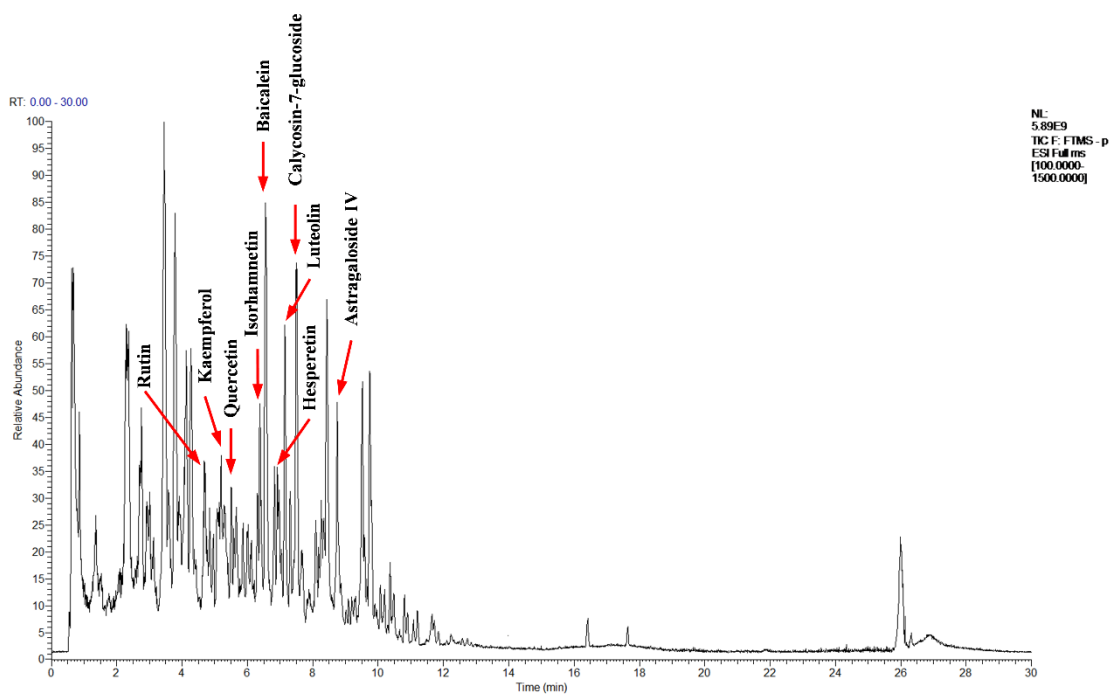
TIC diagram of UHPLC-Q Exactive-MS detection of YJHD granule aqueous solution in negative ion mode.
