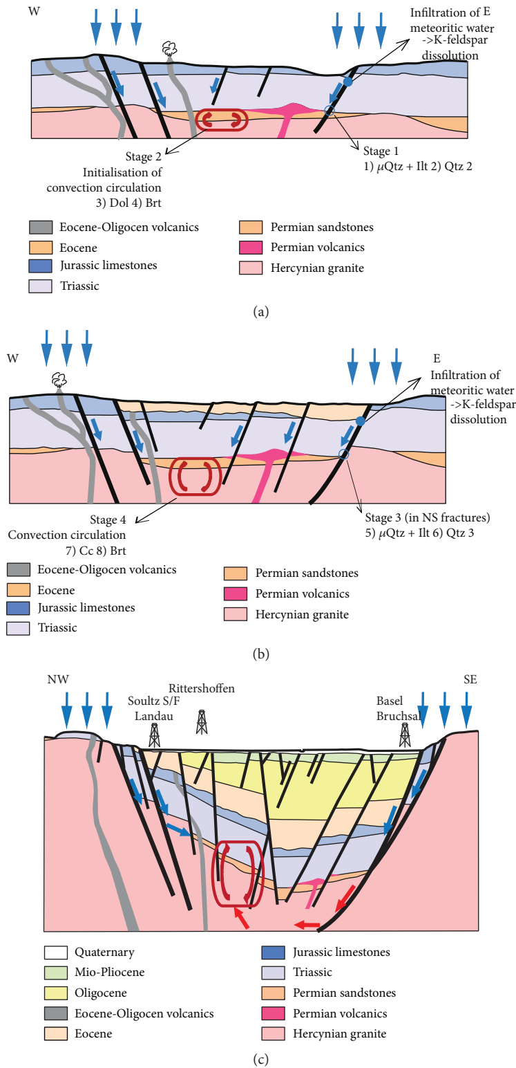
FIGURE 15: Schematic of fluid circulation and rock interaction during Tertiary tectonic episodes. (a) Early rifting stage during the Eocene under N-S compression associated with the paleofluid stages 1 and 2. (b) Lower Eocene and Oligocene rifting under E-W extension associated with paleofluid stages 3 and 4. (c) Present-day situation; location of geothermal sites is indicated as an approximate projection. Conceptual cross sections modified from Sittler (1992). Vertical scale is exaggerated. Blue arrows: meteoritic waters; red arrows: hot brines; curved arrows: convection cell. See explanation in the text.
