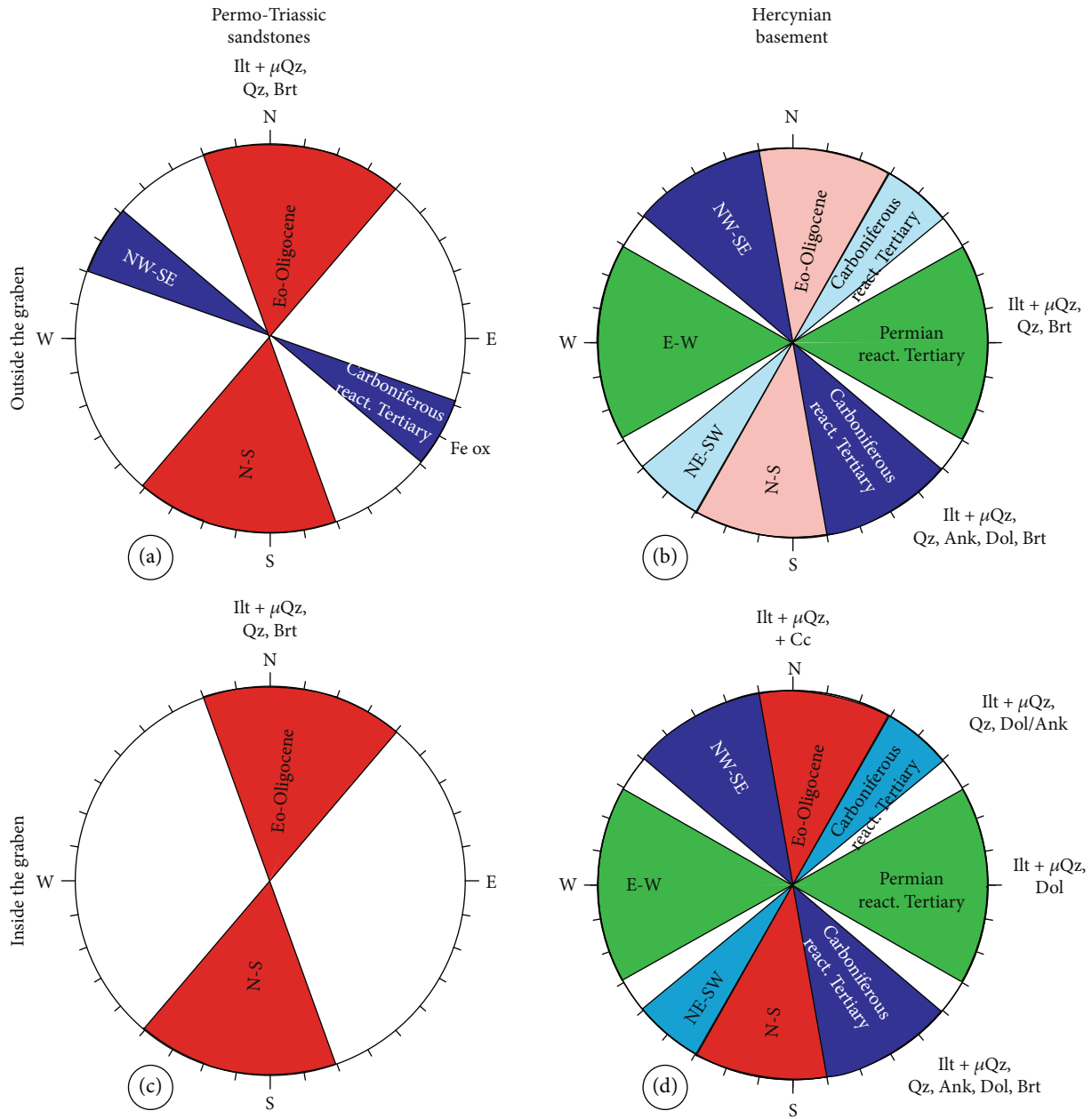
FIGURE 14: Synthesis of the main observed fracture directions with associated filling in the Hercynian granite and the Permo-Triassic sandstones inside and outside the graben. The \text{Ilt} + \mu\text{Qz} combination is generally associated with cataclasis.
