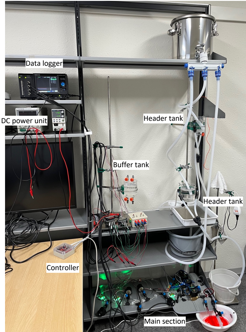
General view
