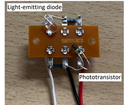
Concentration sensor
