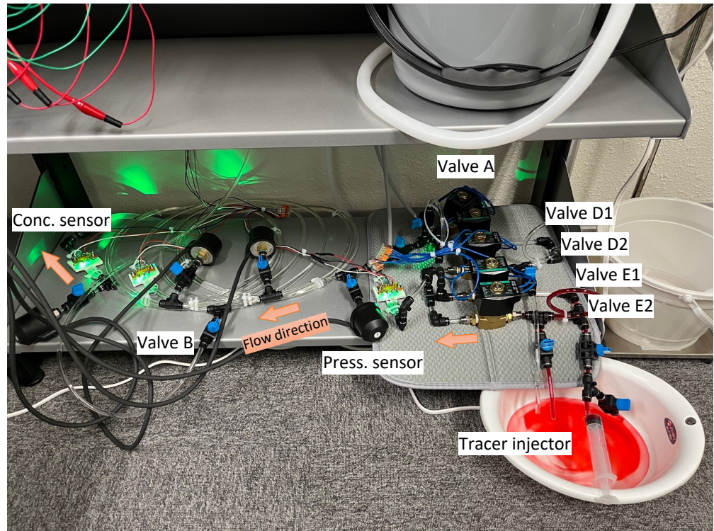
Main section
