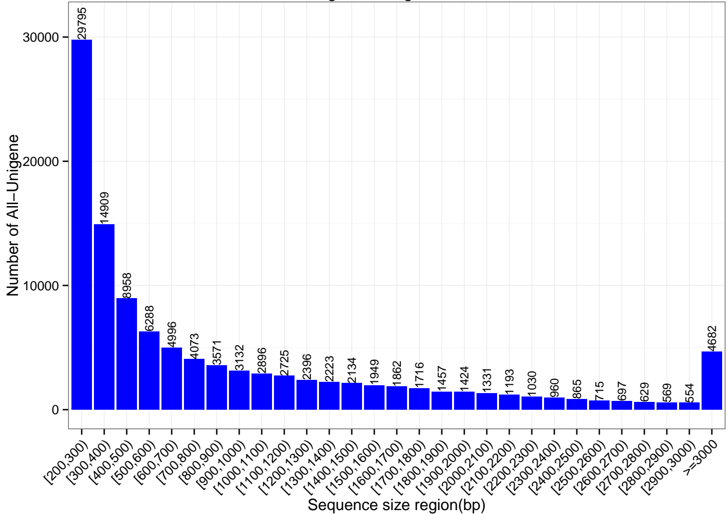
All-Unigene Length Distribution
