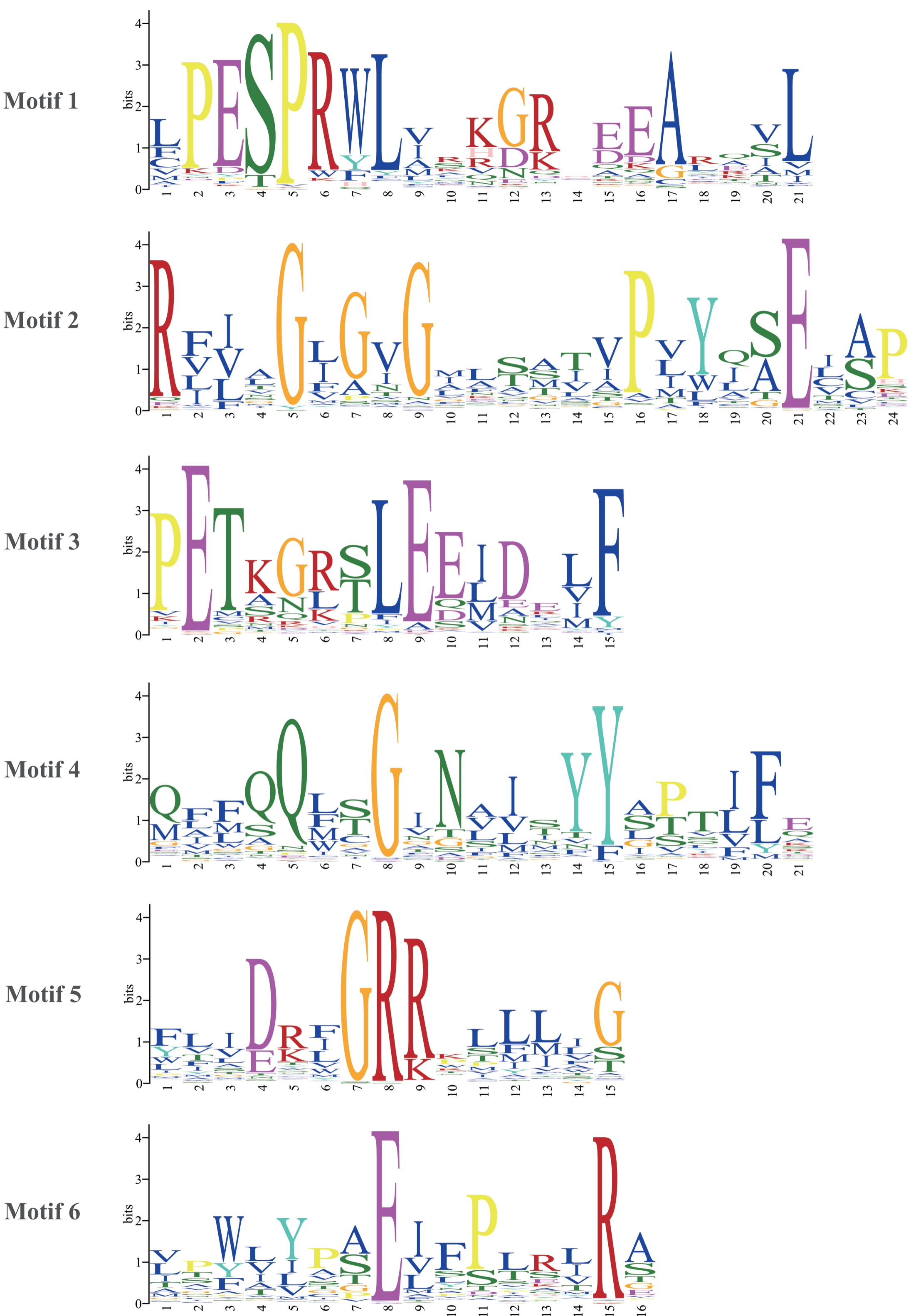
Figure S2: Sequence logos for 6 motifs of sugar transporter (SUT) domains using the MEME program. MEME motifs are displayed by stacks of letters at each site. The total height of the stack is the ‘information content’ of that site in the motif in bits. The height of each letter in a stack is the probability of the letter at that site multiplied by the total information content of the stack. Abscissa represents the width of the motif and ordinate represents the bits of each letter, separately;
