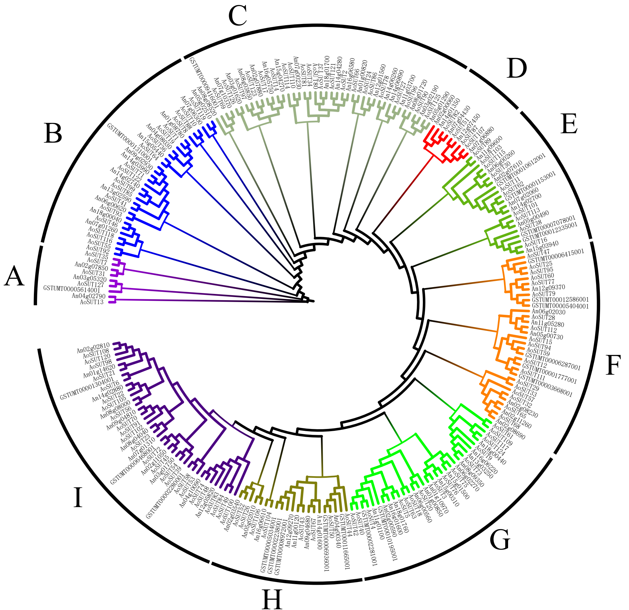
Figure S4: The phylogenetic relationship between A. oryzae , A.niger and Tuber melanosporum SUT proteins. The maximum likelihood tree was constructed by the MEGA X with 1 000 bootstrap replications. Nine clades were distinguished in different colors.
