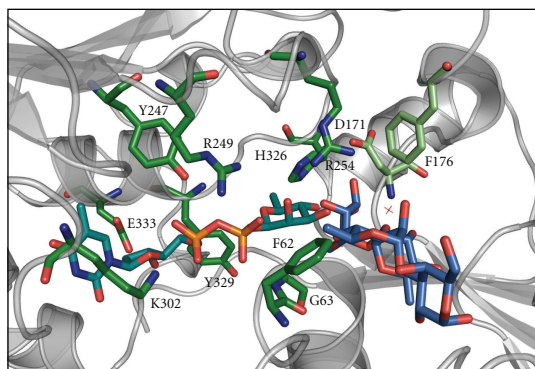
FIGURE 6: Close-up view of WsaF with dTDP- \beta -L-Rha bound in the binding pocket and tri-rhamnose galactose modelled into the putative acceptor binding tunnel. Colour code: turquoise, dTDP-Rha; blue, tri-rhamnose galactose.
