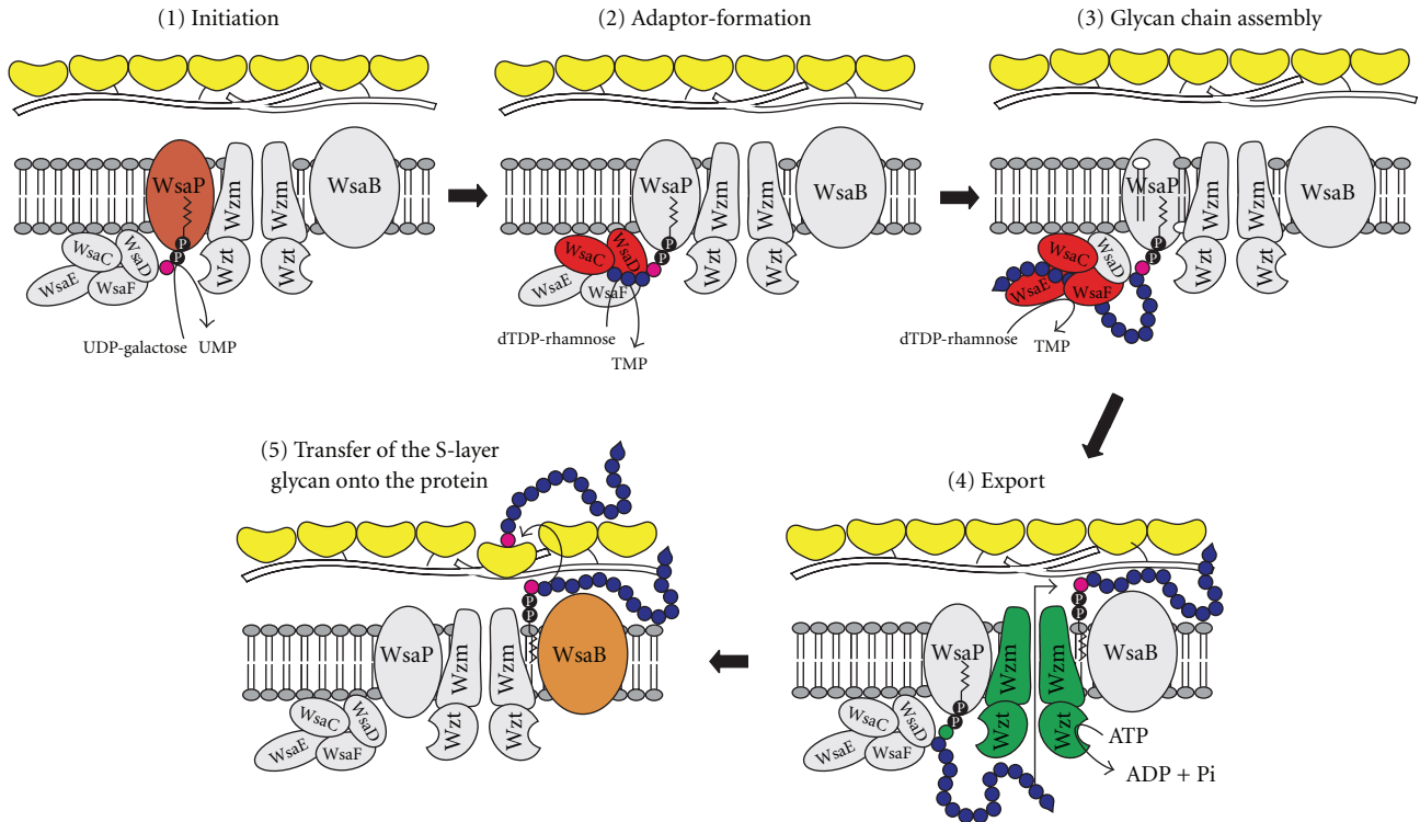
FIGURE 4: Proposed model of S-layer glycoprotein glycan biosynthesis in G. stearotherophilus NRS 2004/3a. (1) Initiation: transfer of a Gal residue from UDP- \alpha -D-Gal to a lipid carrier catalyzed by WsaP. (2) Adaptor formation: \alpha 1,3-linkage of a rhamnose residue from dTDP- \beta -L-Rha to the primer by the action of WsaD, followed by the transfer of one or two additional \alpha 1,3-linked rhamnoses by the action of WsaC. (3) Glycan chain assembly: formation of repeating unit-like structures by action of the rhamnosyltransferases WsaE and WsaF, whereby WsaE is forming the \alpha 1,2- and the \alpha 1,3-linkages, and WsaF is forming the \alpha 1,2-linkage. Shown is termination of chain growth by 2-O-methylation of the terminal repeating unit, catalyzed by the O-methyltransferase domain of WsaE. (4) Export: the Wzt component of the Wzm/Wzt ABC transporter system is predicted to be responsible for binding of the 2-O-methylated glycan chain and its subsequent export through the membrane. (5) Transfer of the S-layer glycan onto the protein: the final transfer of the completed S-layer glycan to the S-layer protein would be catalyzed by the oligosaccharyltransferase WsaB. This research was originally published in the Journal of Biological Chemistry [35]. The American Society for Biochemistry and Molecular Biology. For colour code see Figure 3; pink, linkage glycoside.
